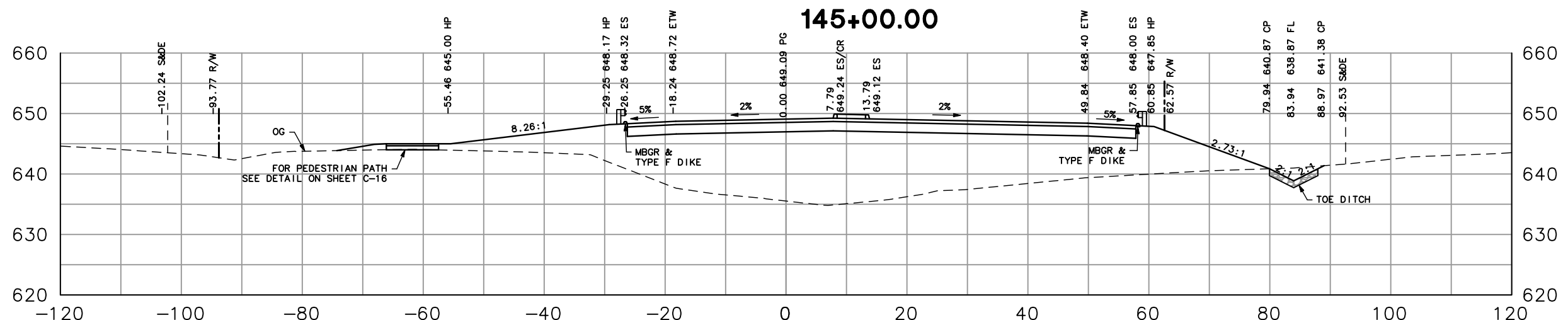
GENERAL CROSS SECTIONS "SVP" LINE SCALE: 1" = 20' 6 OF 38 11/21/2012
