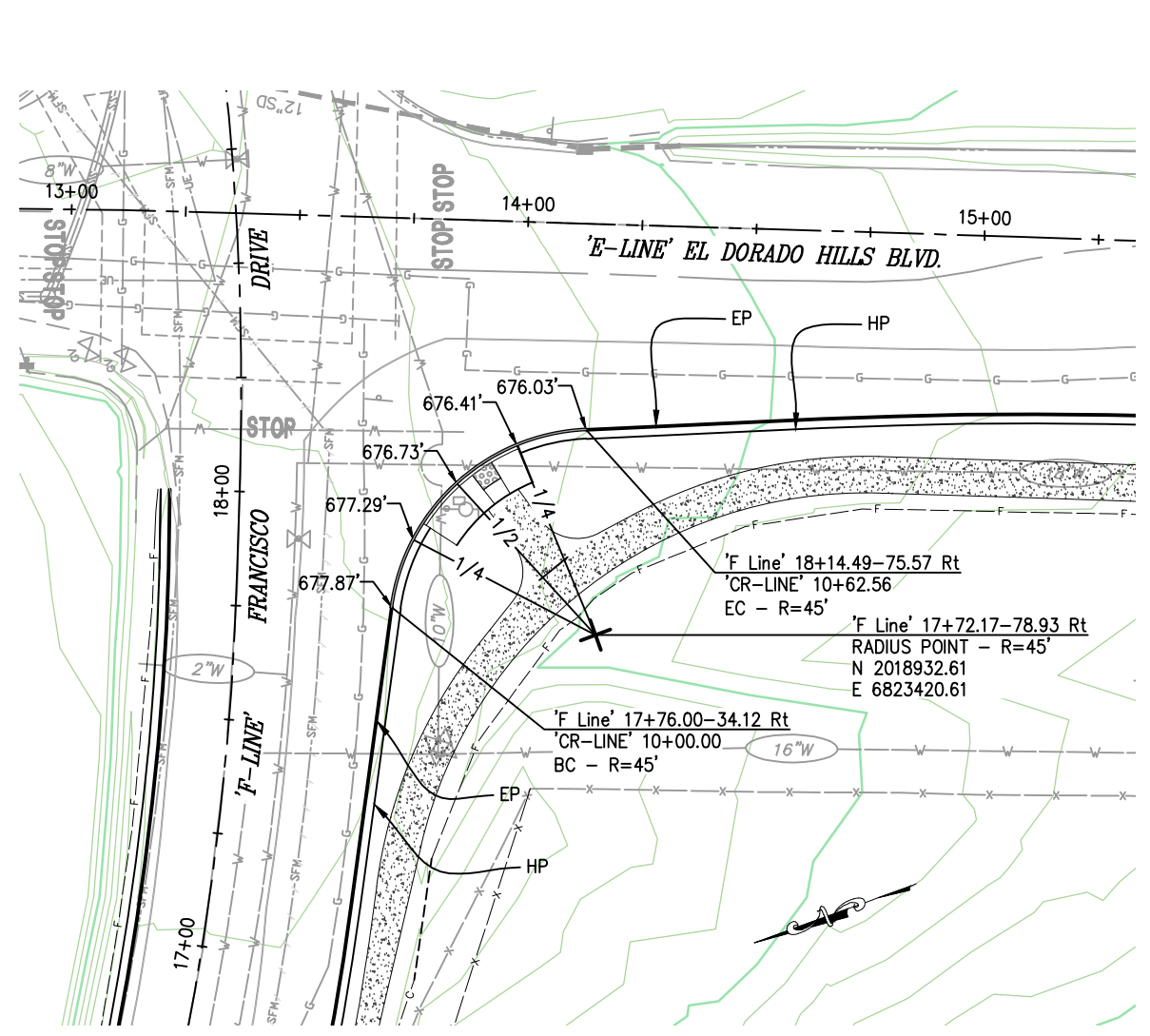
1 CURVE RETURN DETAIL SCALE: 1" = 20'
