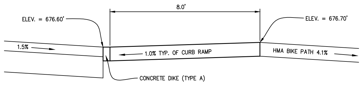
CENTERLINE OF CURB RAMP NO SCALE
