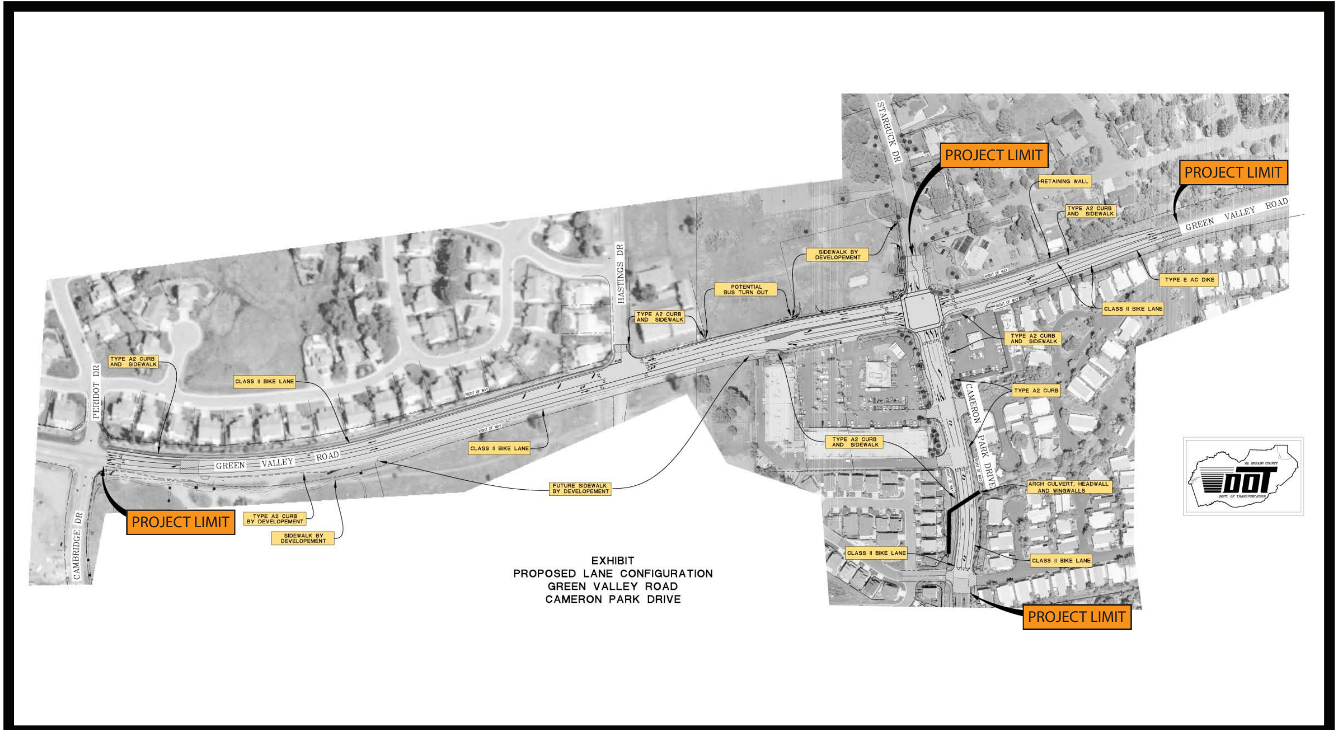
FIGURE 2 Cameron Park Drive/Green Valley Road Intersection Improvements Project Proposed Project
